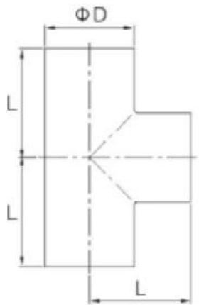
Standard: 3A(Short Equal Weld Tee)
