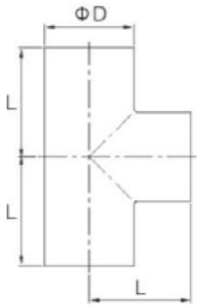
Standard: AS1528(Short Weld Tee)
